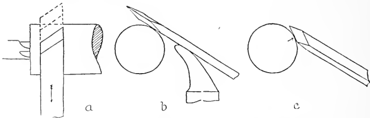
FIG. 298. SUCCESSIVE PLACINGS OF SKEW FOR POSITION.
